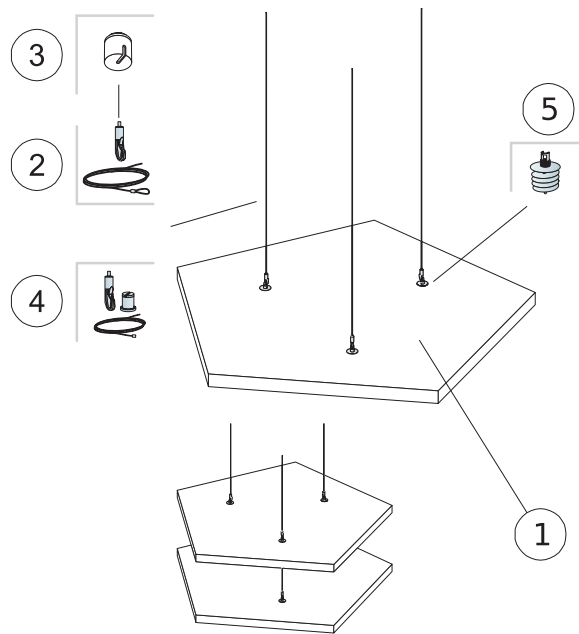
Installation diagram (M427) for Ecophon Solo Pentagon
