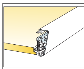
Connection between T-profile and Edge extrusion
