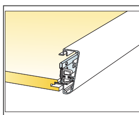
Joint between tile and Edge profile
