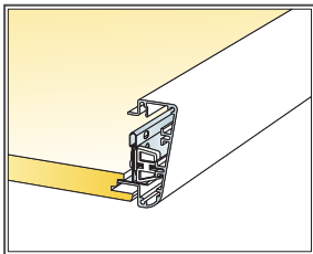
Joint with tile side Ds1
