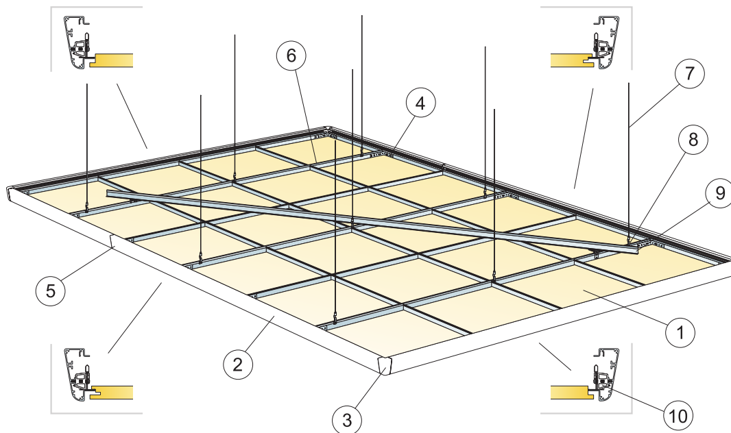
© Saint-Gobain Ecophon AB Installation diagram (M211) for Ecophon Edge 500 with Focus Dg
